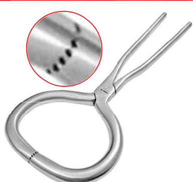
HOOF TESTER ROUND MODEL (DROP FORGED STAINLESS STEEL)
