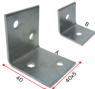
ANGLE BRACKET Size MM
