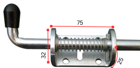
SPRING LATCH 12MM UNIVERSAL
