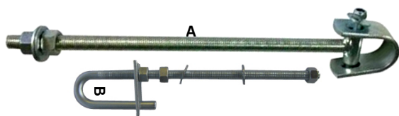
ADJUSTABLE TOP SWIVEL GUDGEON
