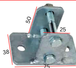
WALL/FLOOR BRACKET FOR PASTURE PANELS
