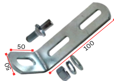
GATE ANGLE BRACKET ADJUSTABLE Size MM
