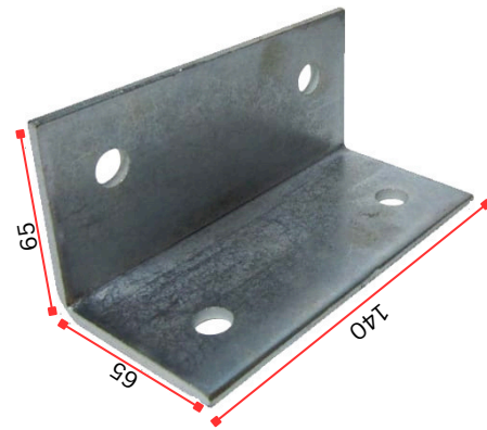
ANGLE BRACKETS Size MM
