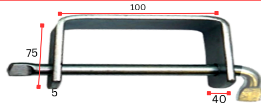
DOUBLE PANEL BRACKET WITH CAPTIVE PIN
