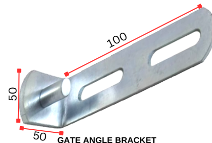
GATE ANGLE BRACKET Size MM
